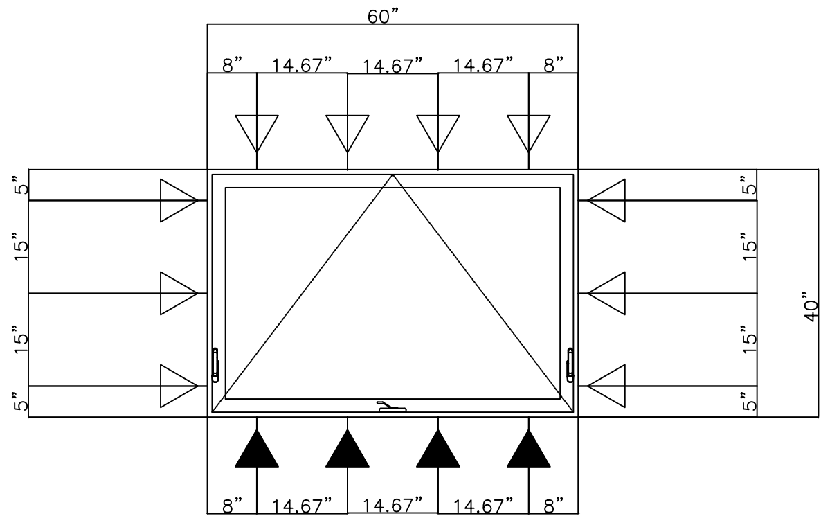
3010i-A4 Single Awning (Impact) – FINLESS INSTALLATION MAXIMUM SIZE 60" X 40" DESIGN PRESSURE +/- 70 PSF MISSILE D – WIND ZONE 4
