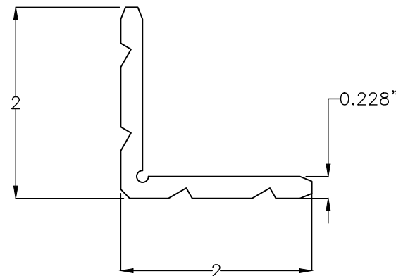
HDW-3669 .968" CORNER KEY MADE FROM #395-222-15V
