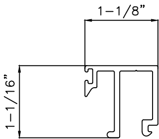
GLAZING STOP 6063-T6
