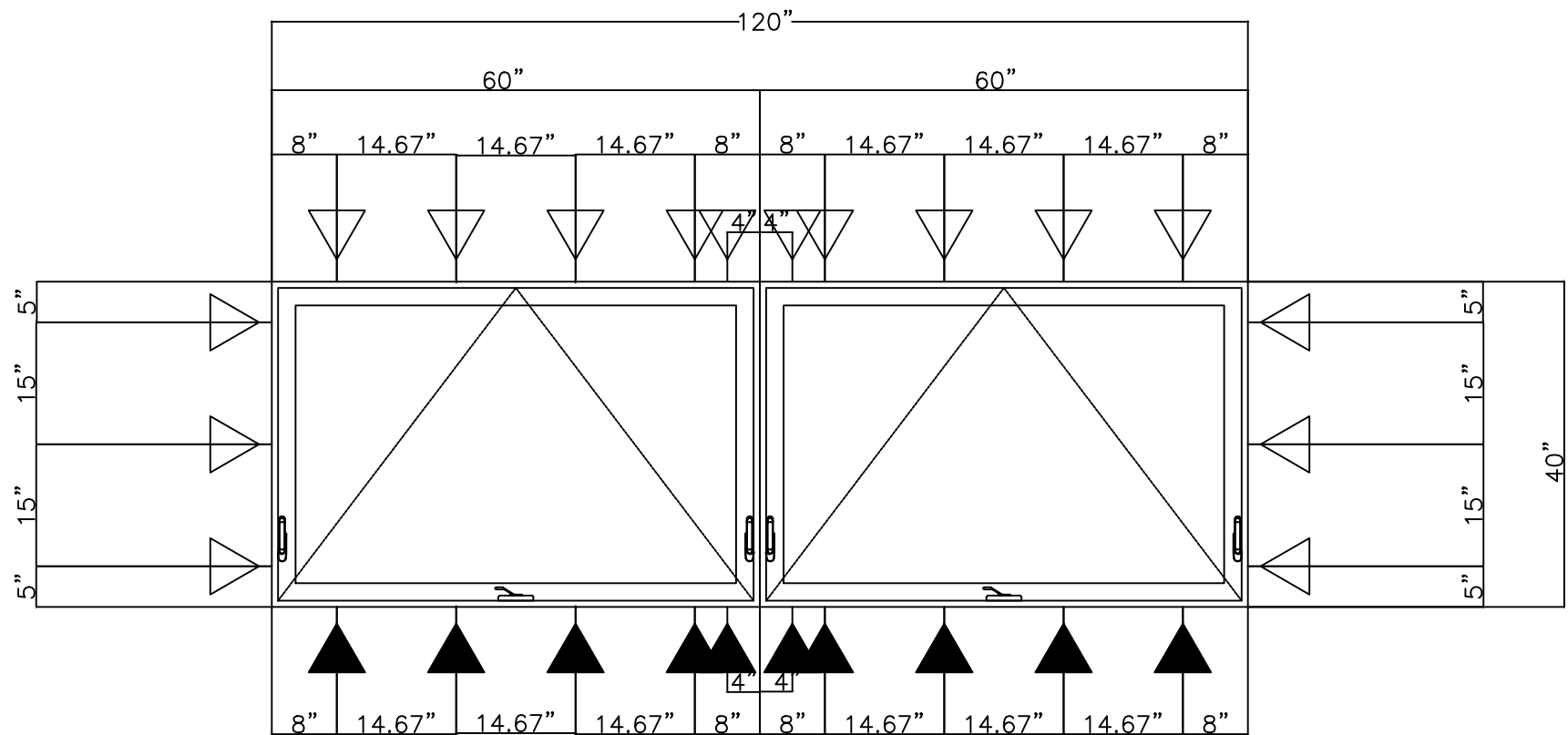
3010i-A4 2-Wide Awning (Impact) – FINLESS INSTALLATION MAXIMUM SIZE 120" X 40" DESIGN PRESSURE +/- 70 PSF MISSILE D – WIND ZONE 4
