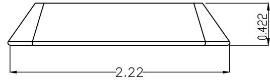
HDW-3691, WEEP COVER ASSEMBLY
