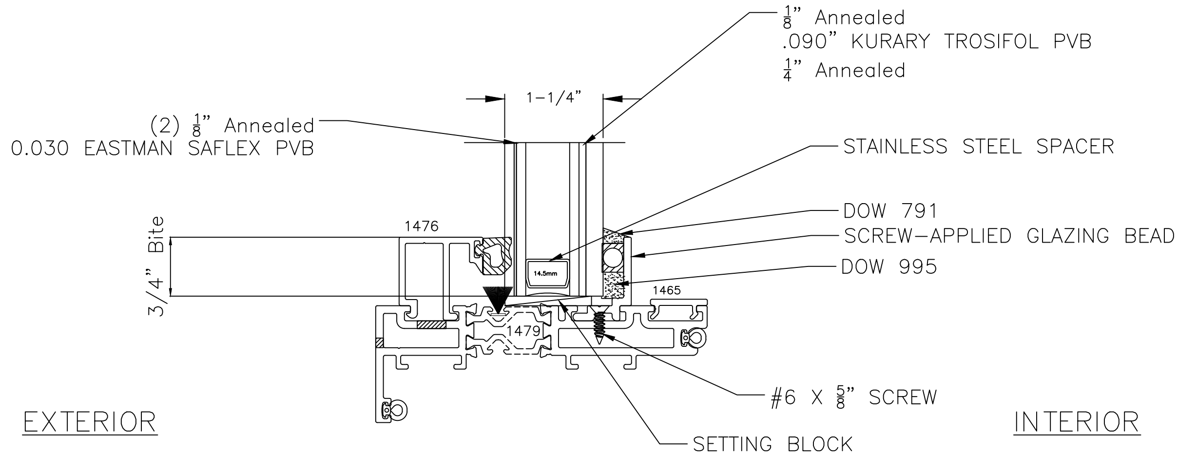
GLAZING DETAIL 1-1/4" INSULATING GLASS
